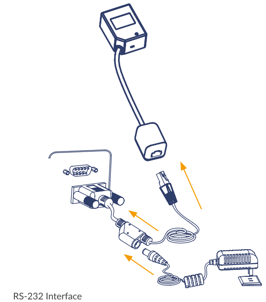
RS-232 Interface
